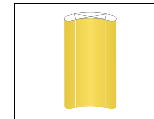
MP1 - 1x3, ref. 82201 820 (a) x 2255 (al) x 200 (f) mm MP2 - 1x3, ref. 82211 1290 (a) x 2225 (al) x 400 (f) mm
